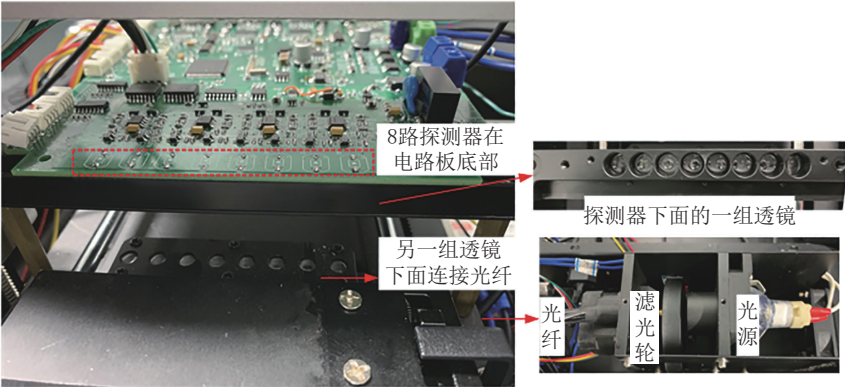
(c) 吸光度检测模块实物图 (c) Physical image of absorbance module
